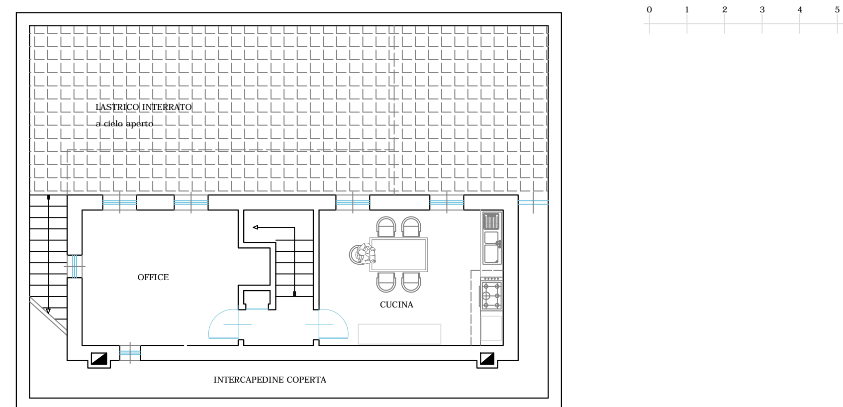
BASEMENT
