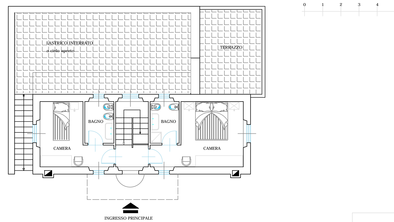
GROUND FLOOR
