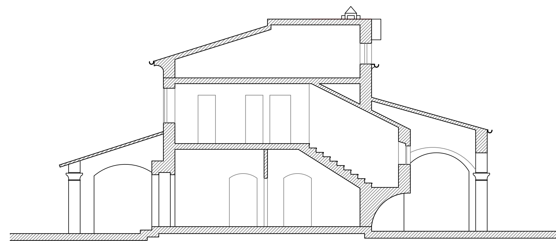
SECTION
